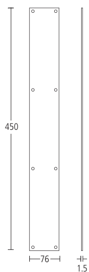
6801G Push plate. Finishes: SS • PS • MA
