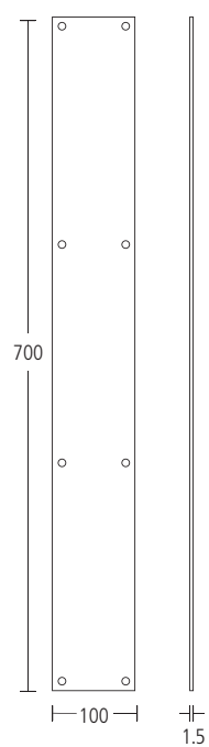
6801K Push plate. Finishes: SS • PS • MA
