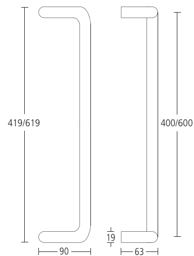
6597CBB Pair, as above, with back-to-back fixings.
