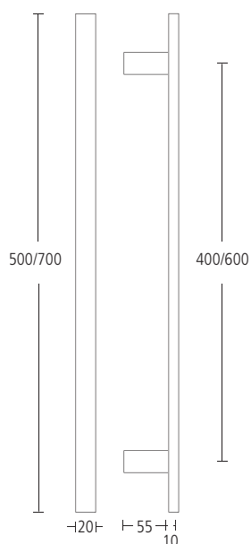
1746BB Pair, as above, with back-to-back fixings
