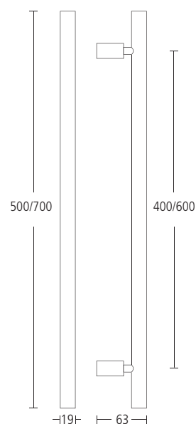
1751BB Pair, as above, with back-to-back fixings
