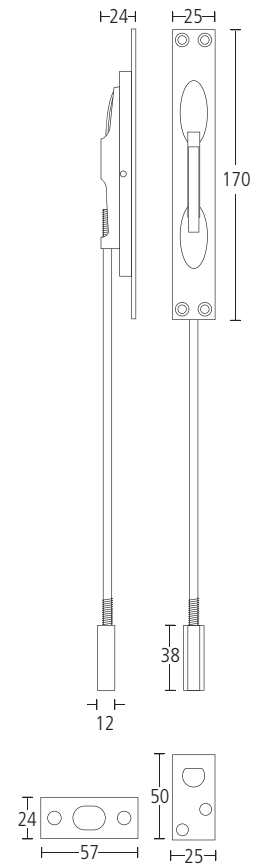
76015SC Lever action flushbolt for metal doors. Finish: XX (Satin chrome)
