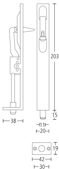
48800 Lever action flushbolt. Finishes: SS • PS
