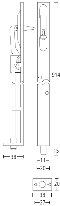
48803 Lever action flushbolt. Finishes: SS • PS
