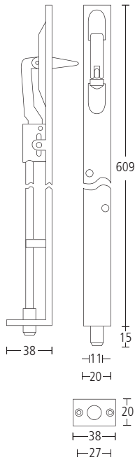
48802 Lever action flushbolt. Finishes: SS • PS
