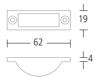
7051 Easy clean flushbolt socket. Finishes: SC • PC
