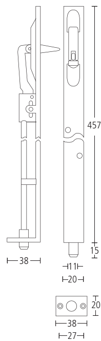
48801 Lever action flushbolt. Finishes: SS • PS
