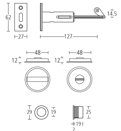
2640 Pocket door locking kit. Finishes: SC • PC
