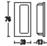
6215 Modric flush pull handle. Finishes: SS • PS • GT • BT • MA
