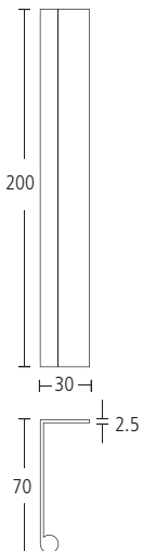
1716/20 As above but with 70mm projection. Finishes: SS (XX1716/2S) PS (XX1716/2P)
