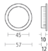
2610 Circular flush pull. Finishes: SC • PC • PB • BB
