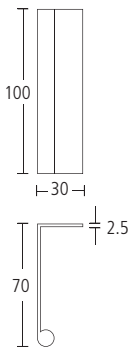
1716/10 As above but with 70mm projection. Finishes: SS (XX1716/1S) PS (XX1716/1P)
