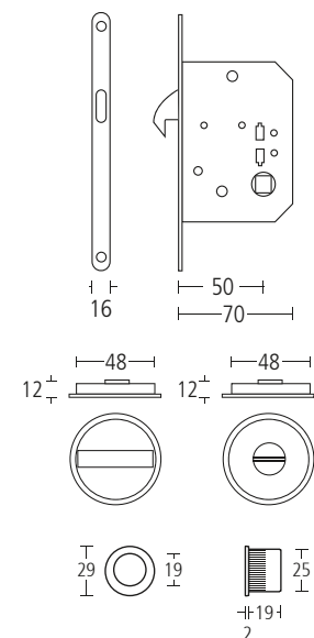
2640 Pocket door locking kit. Finishes: SC • PC
